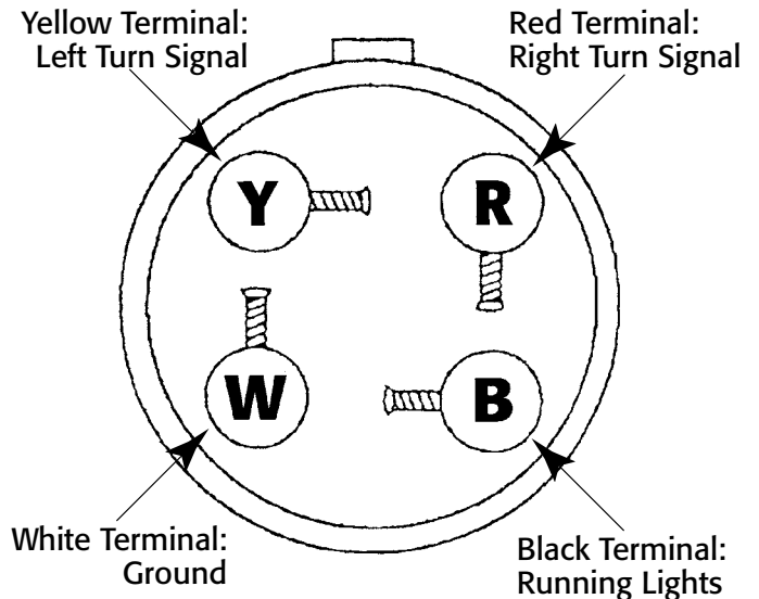
Magnetic Towing Light Connector Schematic
